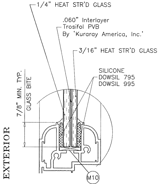
GLAZING DETAIL
