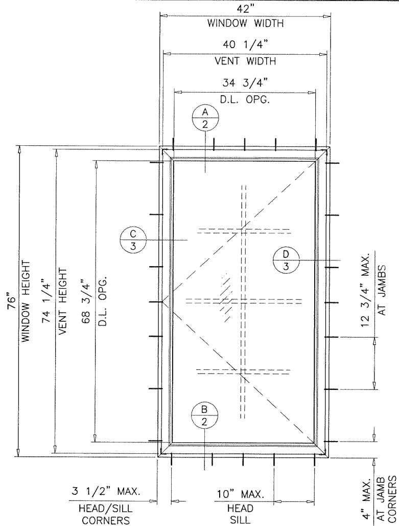
TYPICAL ELEVATION
